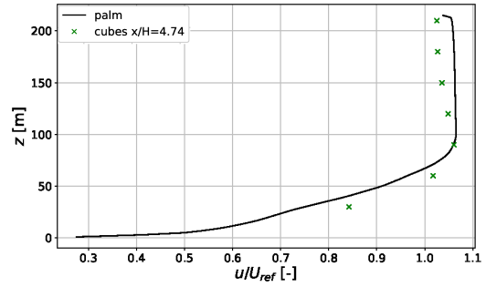
Fig. 14: Velocity profile compared to empty tunnel with roughness elements only (cubes).
