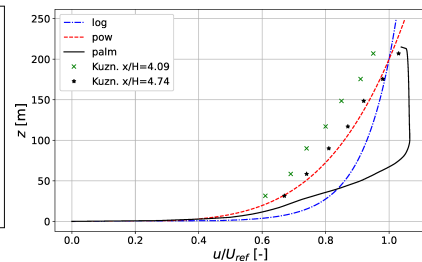
Fig. 9: Velocity profiles at the beginning of the test section.
