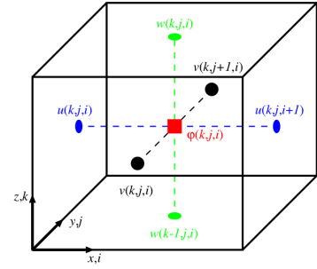
Fig. 1: Arakawa staggered C-grid [4]
