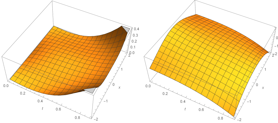
FIG. 3.1. Solutions from left: y_1(x,t) , y_2(x,t) , \tau = 0 .
