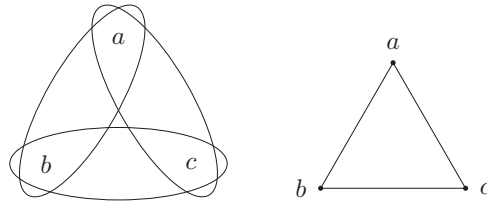
FIG. 2.1: The left depicts the three point space X := \{a, b, c\} equipped with the cover \lambda := \{\{a, b\}, \{a, c\}, \{b, c\}\} . The right depicts a geometric realisation of \mathcal{V}(X, \lambda, \in) within the plane.
