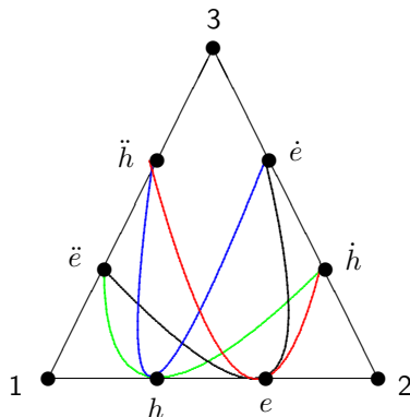
Fig. 1. Geometric representation of Dow_3(C_2) .
