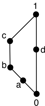
Fig. 1. (L, \preceq) .
