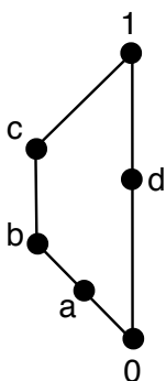
Fig. 3. (L, \preceq_{U_2})
