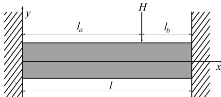
Fig. 5. Point load.
