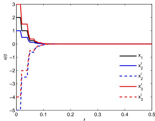
Fig. 3. Trajectories of real and imaginary parts of x_i(t) with impulse.
