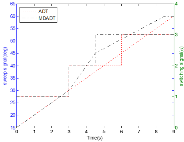
Fig. 6. Sweep angle and switching signal.
