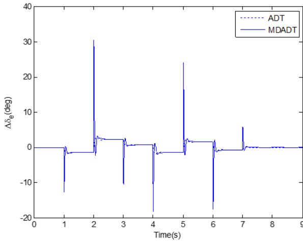
Fig. 9. Elevator deflection.
