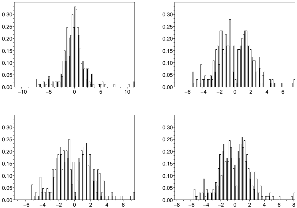
Fig. 1. DAX daily data set, top left: original data, top right: data transformed with the parameters obtained by the M_1 technique, bottom left: data transformed with the parameters obtained by the M_2 technique, bottom right: data transformed with the parameters obtained by the GMLE technique.
