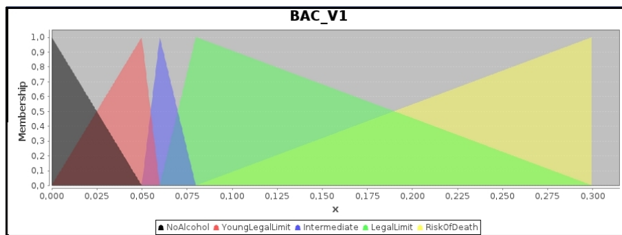
Fig. 2. The ideal fuzzy partition for the BAC example.
