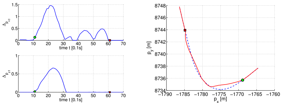
Fig. 3. Courses of absolute estimation errors \Delta p_{x;t} and \Delta p_{y;t} for an experiment with unsatisfactory results (left) and respective part of trajectory (right) with marked beginning (circle) and end (square) of the data outage where full line is the estimated trajectory, dashed line is the true trajectory.
