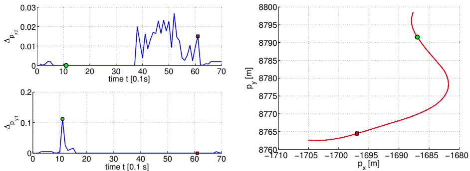
Fig. 2. Courses of absolute estimation errors \Delta p_{x;t} and \Delta p_{y;t} for an experiment with satisfactory results (left) and respective part of trajectory (right) with marked beginning (circle) and end (square) of the data outage.
