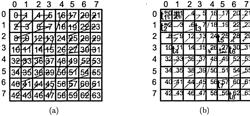
Fig. 1. a) The Z-curve filling the entire 2-dimensional space 8 \times 8 . b) 2-dimensional space 8 \times 8 with tuples t_1 - t_8 . These tuples define the BUB-tree Z-regions partitioning [0:2],[7:11],[25:30],[57:62] with the node capacity 2.
