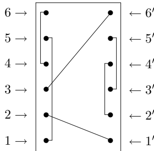
Figure 1. The element \{\{1, 5\}, \{4, 6\}, \{2', 4'\}, \{3', 5'\}, \{2, 1'\}, \{3, 6'\}\} of \mathfrak{B}_6 .
