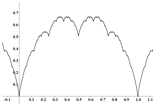
Figure 1. Takagi's function
