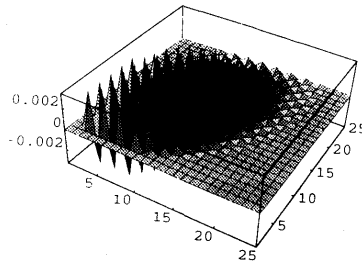
Fig. 12. Impulse Response of a 2-D system with B(z_1, z_2) = 1/\tilde{f} .
