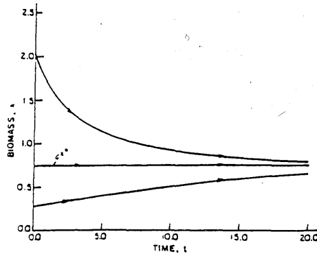
Fig. 1. Harvested one species system, undisturbed and uncontrolled.
