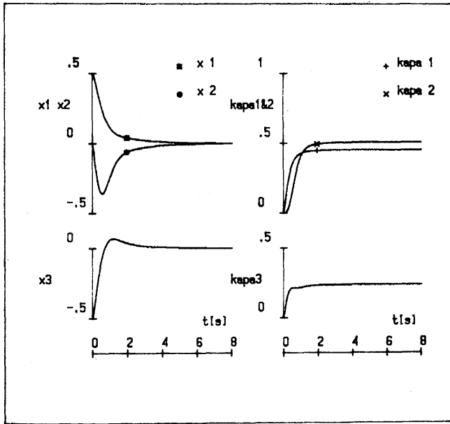
Fig. 3. Systems responses, adaptive control law (34.b).
