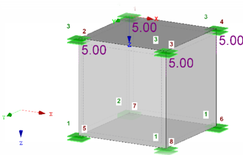
Figure 1: Benchmark model.
