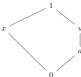
Fig. 2. Lattice diagram of L
