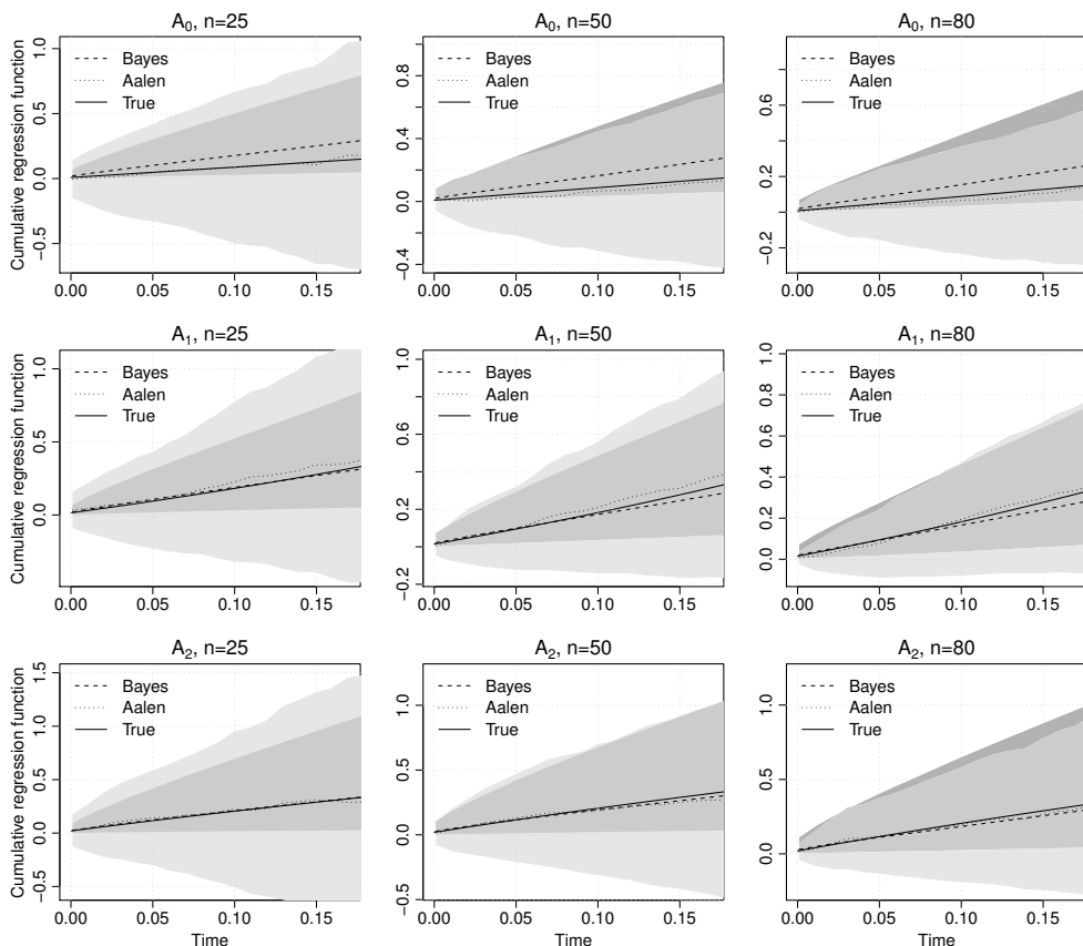
Fig. 1. Graphs of the pointwise averages of the estimators obtained from 100 repetitions for prior 1 and numbers of observations n = 25, 50 and 80 . The true regression function is plotted in solid line, average of the Bayesian estimators in dashed line and average of the Aalen’s estimators in dotted line. The average pointwise credibility/confidence bands are included: Bayesian credibility bands in dark gray and Aalen’s confidence bands in light gray.
