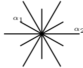
FIG. 1: The root system of Lie G_2
