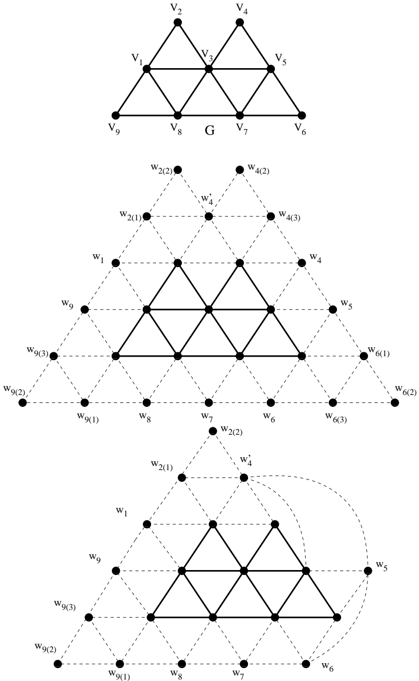
FIGURE 3. The graph G \in \mathcal{G}(4, 0, 1) is “wrapped” to the graphs C(G) and C_T(G) (where T = \{v_4, v_6\} ).
