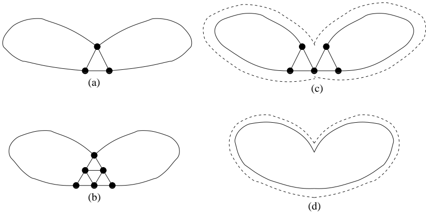
FIGURE 6. The four cases of Lemma 13.
