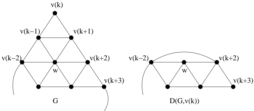
FIGURE 2. Removing external vertices of degree 2 via the operation D .
