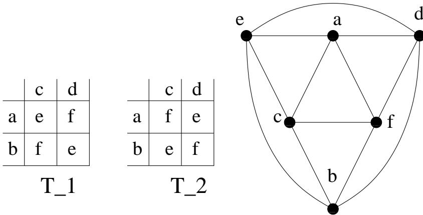
FIGURE 1. The unique 4-regular planar Eulerian triangulation and its corresponding Latin bitrade \{T_1, T_2\} .
