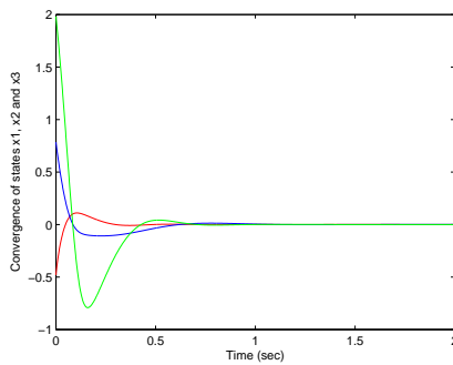
Fig. 16. Convergence of states x_1 (red line), x_2 (blue line) and x_3 (green line) to zero for the Lorenz model.
