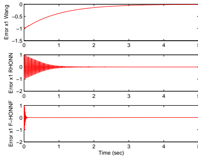
Fig. 8. Approximation Error of variable x_1 for Wang, RHONN and F-HONNF approach.
