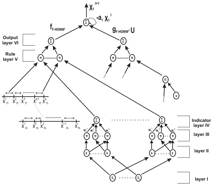
Fig. 1. Configuration of a neuro-fuzzy (F-RHONN) approximator.
