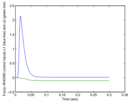
Fig. 15. Evolution of u_1 and u_2 for Fuzzy-RHONN Model.
