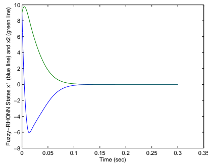
Fig. 13. Convergence of x_1 and x_2 to zero for Fuzzy-RHONN Model.
