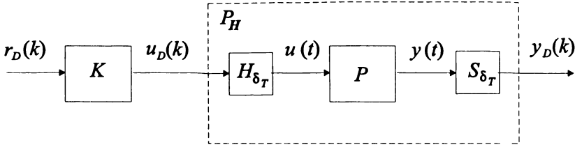
Fig. 1. The hybrid control system S .
