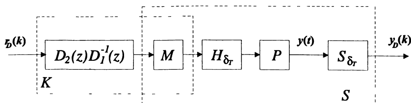
Fig. 4. Factorisation of compensator K .
