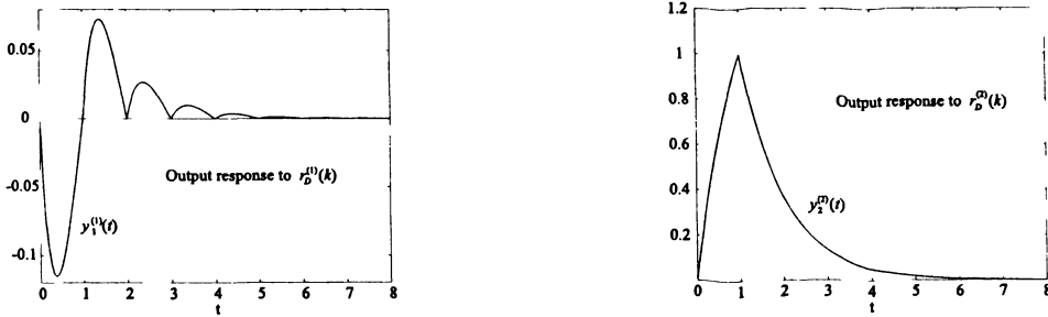
Fig. 2. The nonzero components of the output responses y^{(1)}(t) and y^{(2)}(t) considered in Example 1.
