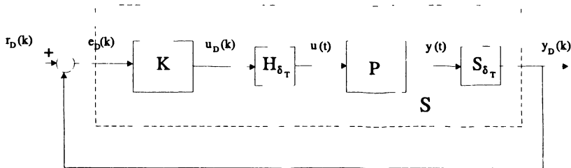
Fig. 3. The hybrid control system \Sigma considered in Proposition 2.
