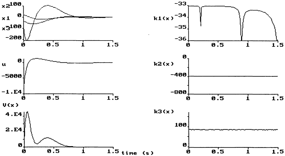
Fig. 4. Uncertain controlled system with \alpha = 6s^{-1} .
