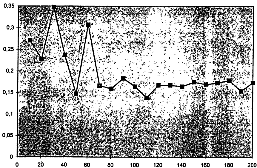
Fig. 12. P_E^{\text{perc}}(n) versus number of learning steps for \Lambda = 1 .
