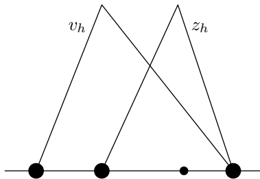
Figure 4. Orthogonality between derivatives of coarse grid basis function v_h and fine grid basis function z_h .
