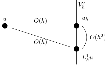
Figure 2. Supercloseness of \nabla u_h and \nabla L_h^1 u when measured in the L^2 -norm.
