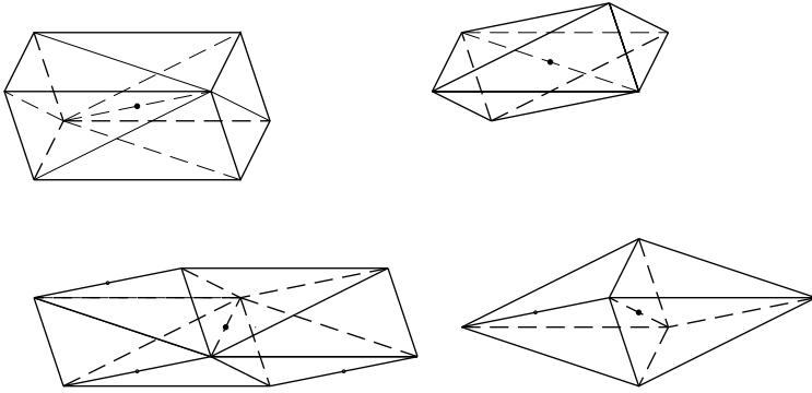
Figure 3. Examples of point-symmetric patches in three space dimensions.
