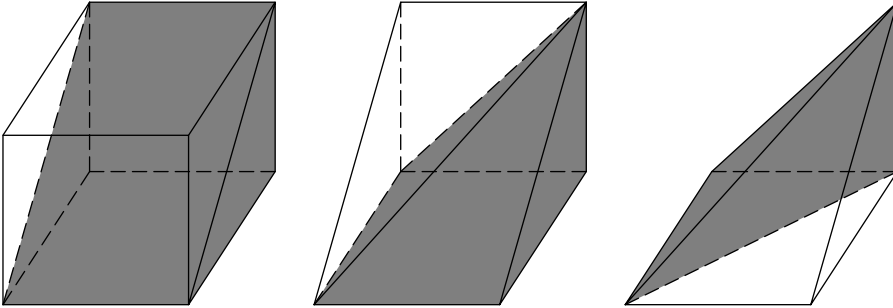
Figure 6. Partition of the cube into six tetrahedra according to (18).
