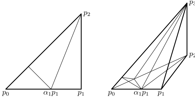
Figure 1. Cutting the path- n -simplex into (n + 1) path-subsimplices. The n -section is the degenerate case that results from letting \alpha_1 tend to one.
