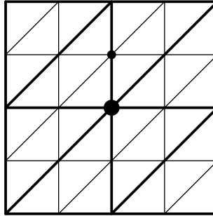
Figure 5. Uniform refinement of a triangulation with (\nabla v_h, \nabla z_h) being non-trivial.
