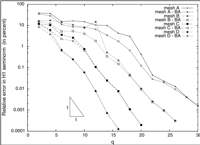
Figure 13. q -convergence of the PUM and the best approximation for the domain \Omega_1 using Mesh A, B, C, and D computed using wave-bands functions.
