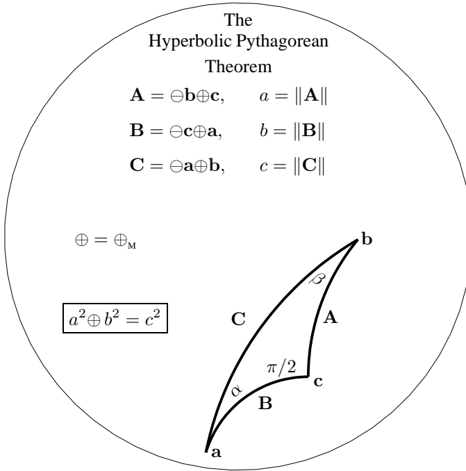
Figure 2: The Hyperbolic Pythagorean Theorem in the Poincaré disc model of hyperbolic geometry that is, equivalently, in the Möbius gyrovector plane (\mathbb{B}, \oplus, \otimes) , \oplus = \oplus_M [22],[23].
