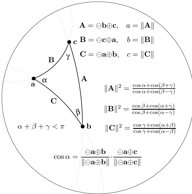
Figure 1: A Möbius triangle \Delta abc in the Möbius gyrovector plane (\mathbb{B}, \oplus, \otimes) , \oplus = \oplus_M is shown. Its sides are formed by geodesic segments that link its vertices \mathbf{a} , \mathbf{b} and \mathbf{c} , having the hyperbolic lengths a, b and c . The cosine of its angles are given by an identity that is fully analogous to its Euclidean counterpart. The Möbius gyrovector plane forms the setting for the Poincaré disc model of hyperbolic geometry just as the common vector plane forms the setting for the standard model of Euclidean plane geometry [13],[23]. Unlike the Euclidean triangle, the sides of the hyperbolic triangle are uniquely determined by its angles.
