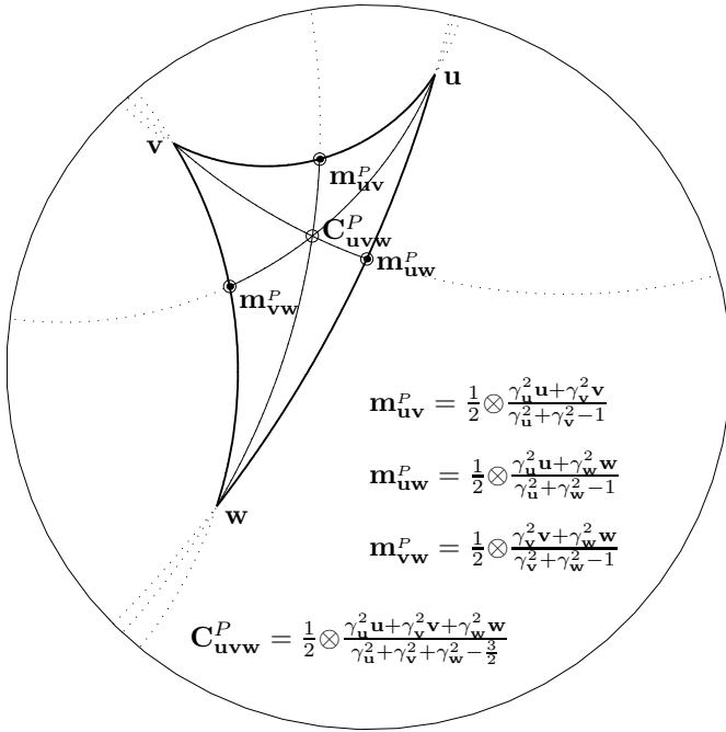
Figure 4: A triangle \Delta uvw in the Poincaré disc model of hyperbolic geometry is shown with the midpoints m_{uv}^P , m_{uw}^P and m_{vw}^P of its sides, and its medians, and centroid C_{uvw}^P .
