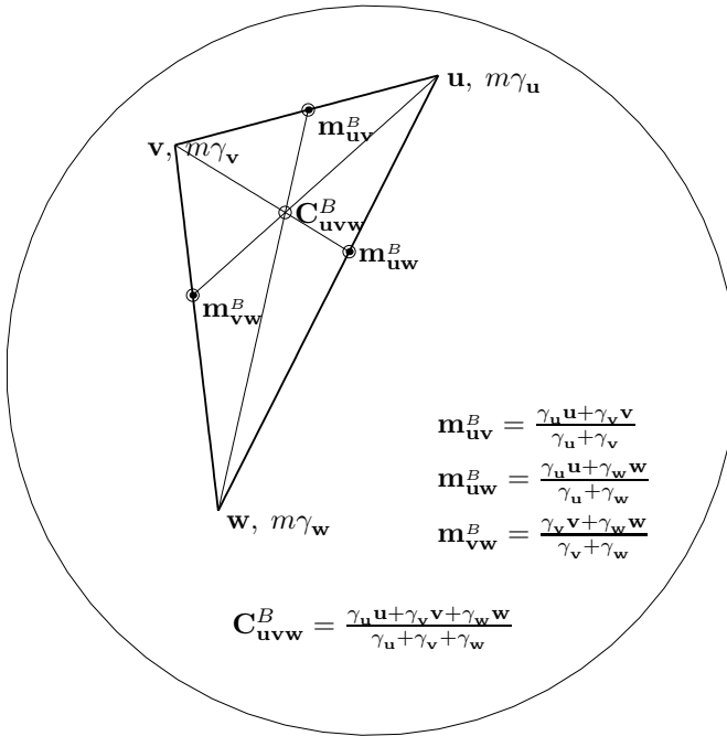
Figure 3: Hyperbolic midpoints, medians and a centroid of a triangle and its sides in the Beltrami model and its underlying Einstein gyrovector space. They possess a relativistic mechanical interpretation, analogous to the classical mechanical interpretation of their Euclidean counterparts in [11],[26].
