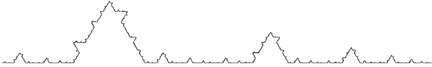
Fig. 1. The attractor von-Koch-infinite
